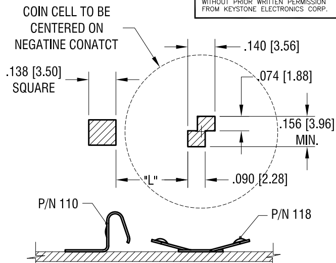
MTG LAY OUT WHEN USE WITH P/N 110
