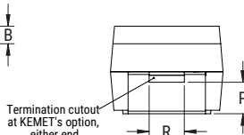
ANODE (+) END VIEW
