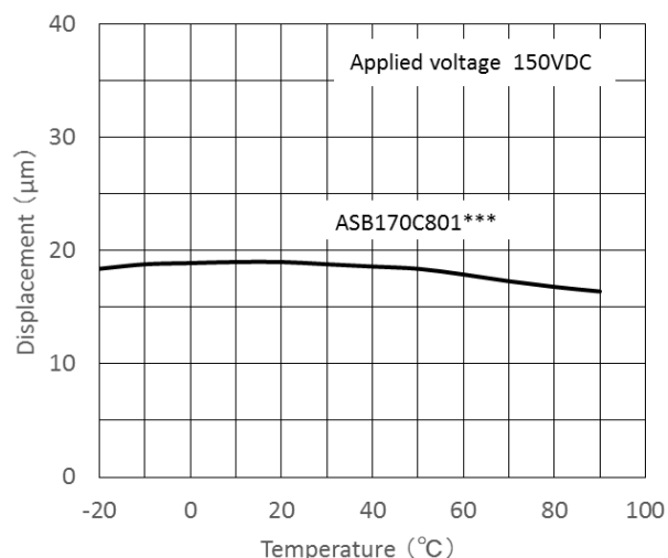
Figure 4 - Temperature vs. Displacement
