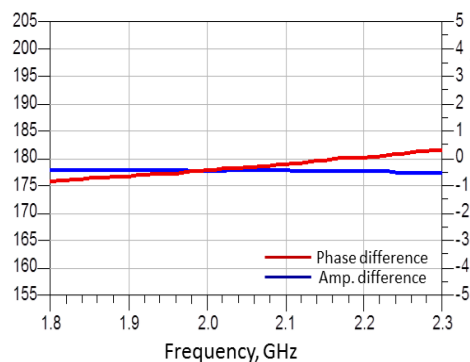
Amplitude and Phase Balance
