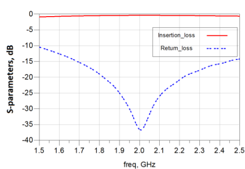
Insertion and Return Loss
