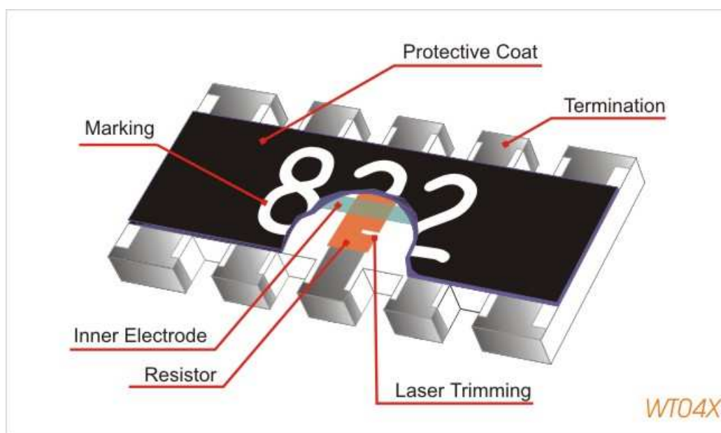
Fig 1. Constuction of a Chip-R network WT04X
