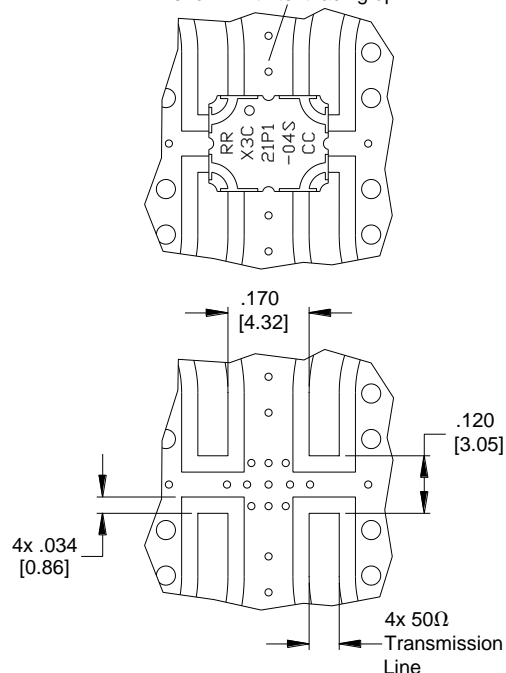
Dimensions are in Inches [Millimeters] X3C21P1-04S Mounting Footprint
