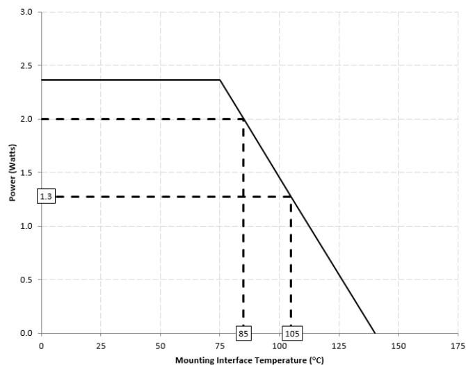
DC2337J5020AHF Power Derating Curve
