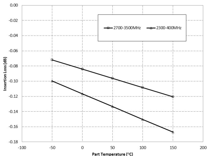
XMC0204E2-03G Typical Insertion Loss Derating Curve
