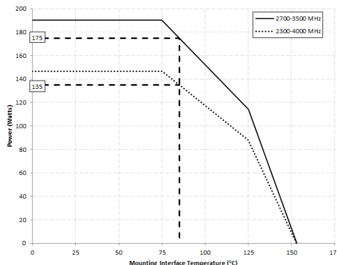
XMC0204E2-03G Power Derating Curve
