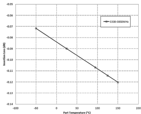
XC3500P-03S Typical Insertion Loss Derating Curve
