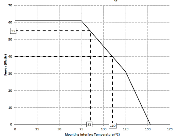
XC3500P-03S Power Derating Curve
