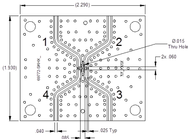
2dB, 3dB, 4dB and 5dB Test Board
