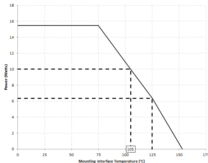
X4C55K1-03S Power Derating Curve
