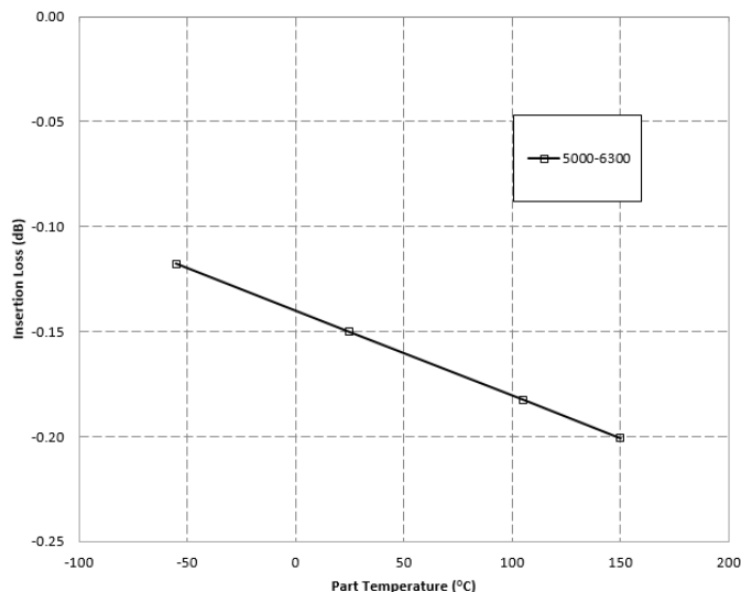
X4C55K1-03S Typical Insertion Loss Derating Curve
