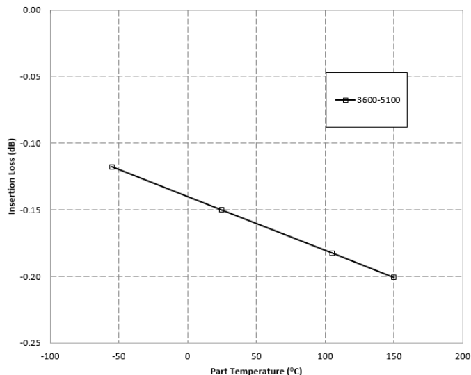
X4C45K1-03S Typical Insertion Loss Derating Curve
