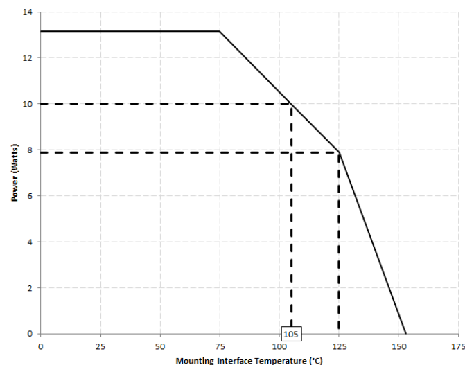
X4C45K1-03S Power Derating Curve
