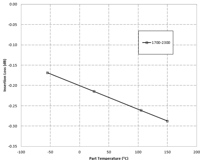
X4C20K1-03S Typical Insertion Loss Derating Curve
