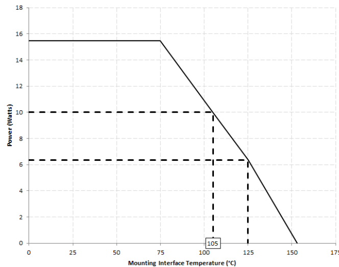
X4C20K1-03S Power Derating Curve
