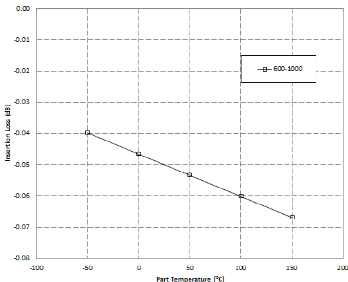
X4C09F1-30S Typical Insertion Loss Derating Curve
