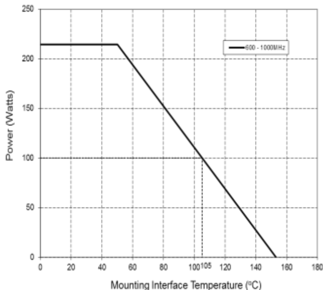
X4C09F1-30 Power Derating Curve
