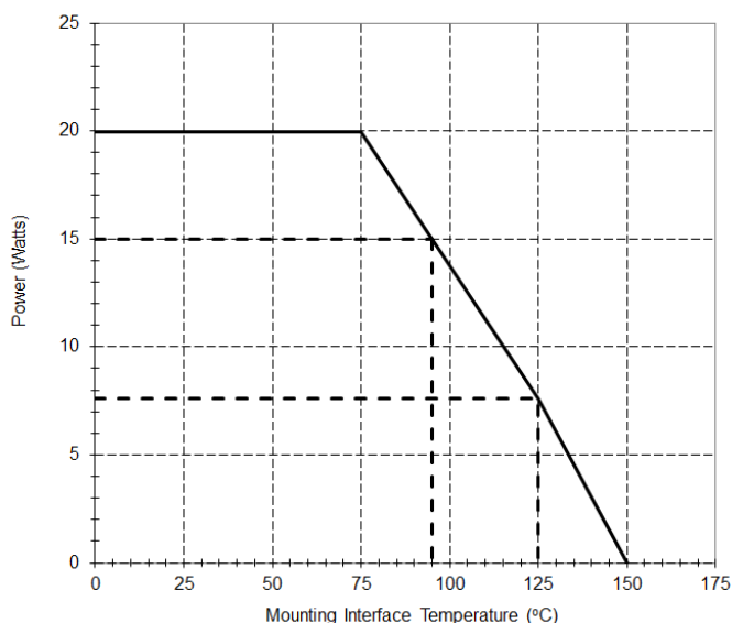
X3C70F1-03S Power Derating Curve
