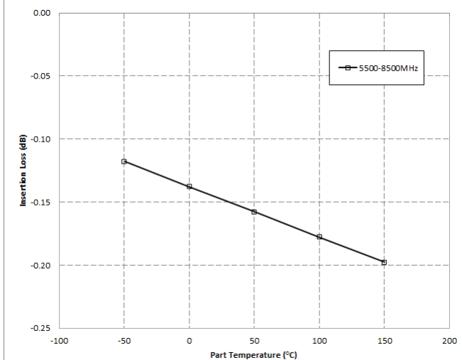
X3C70F1-03S Typical Insertion Loss Derating Curve
