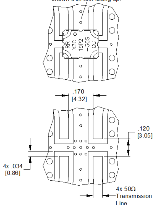
Dimensions are in Inches [Millimeters] X3C19P2-30S Mounting Footprint
