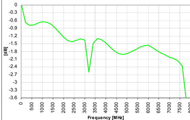
Insertion Loss
