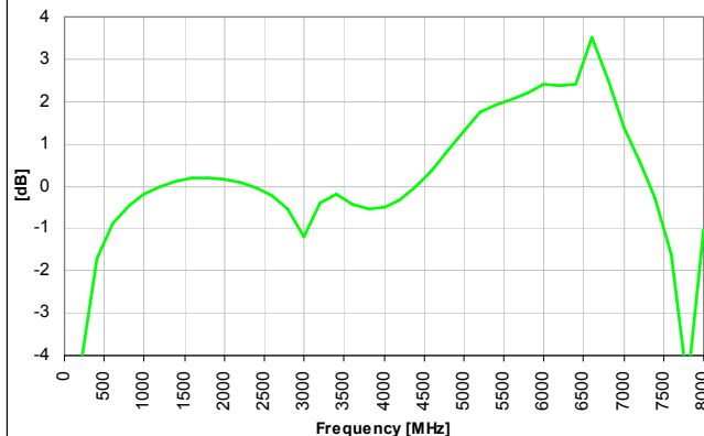
Amplitude Balance
