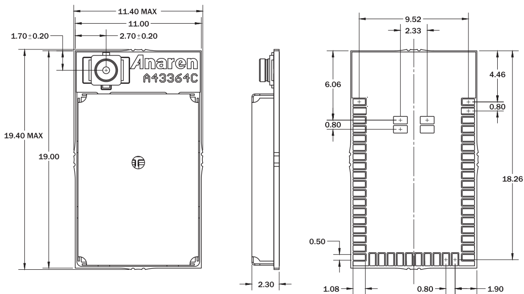
Figure 9: A43364C Dimensions
