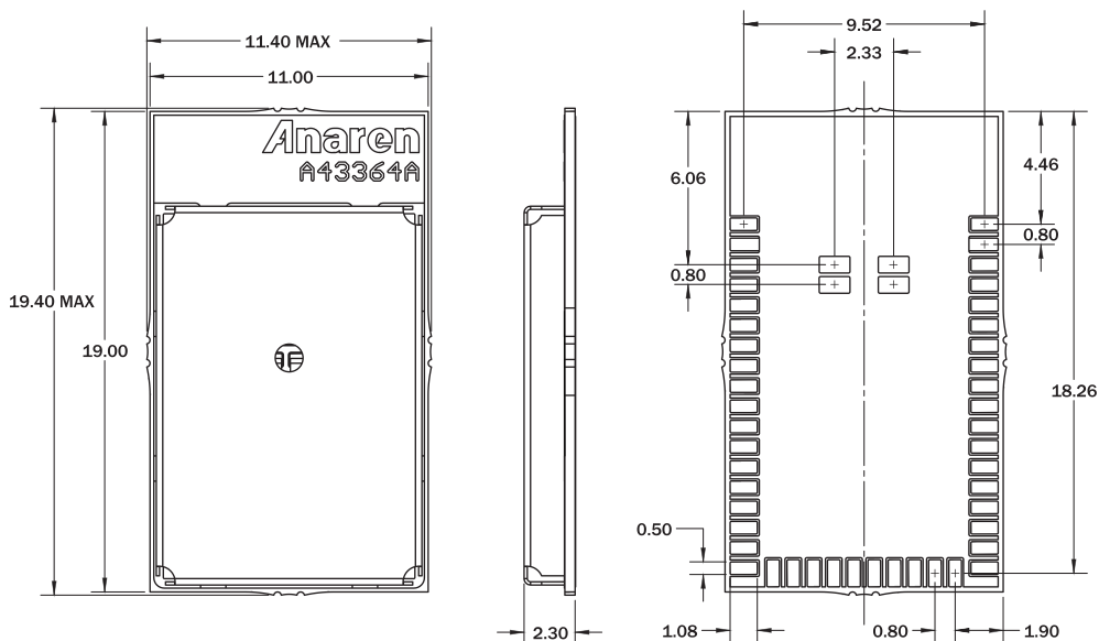
Figure 8: A43364A Dimensions
