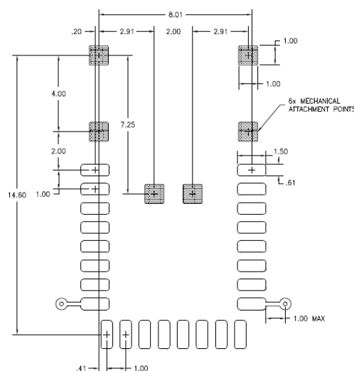
Footprint (PWB)
