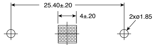
PBC Mounting Layout
