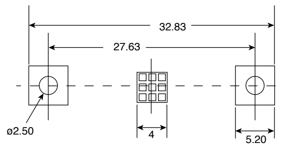
PBC Mounting Layout
