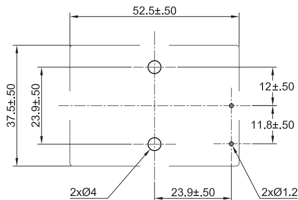
PCB/MOUNTING LAYOUT
