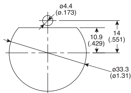
Panel Cut-Out
