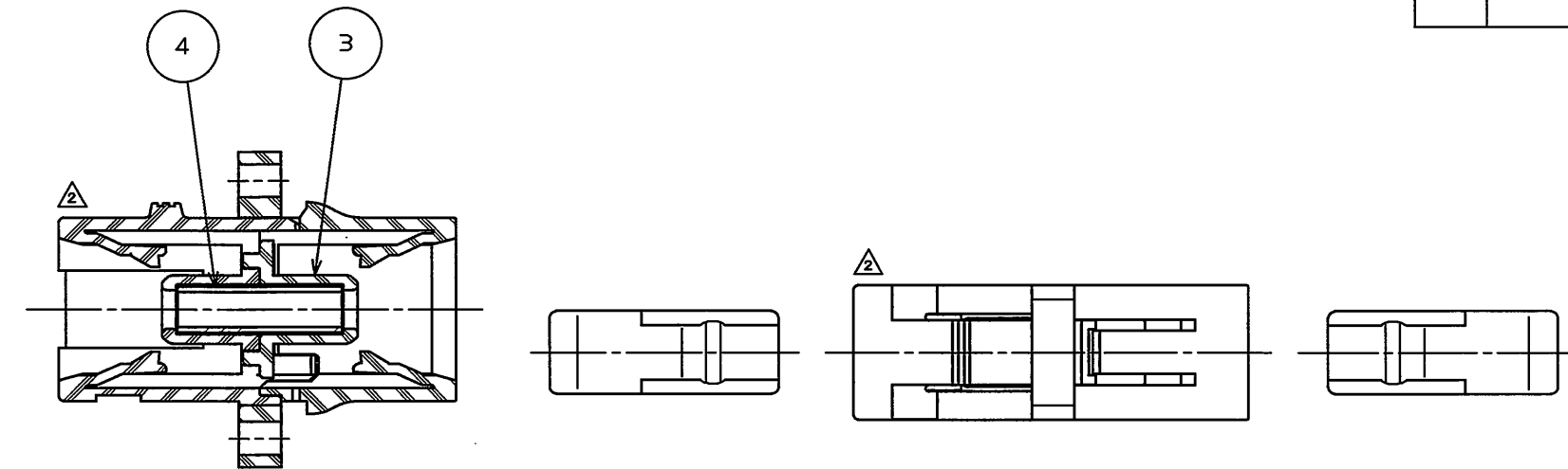
SECT. A-A
