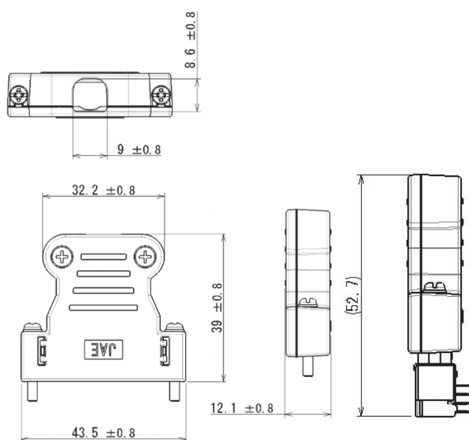
Mated Condition
