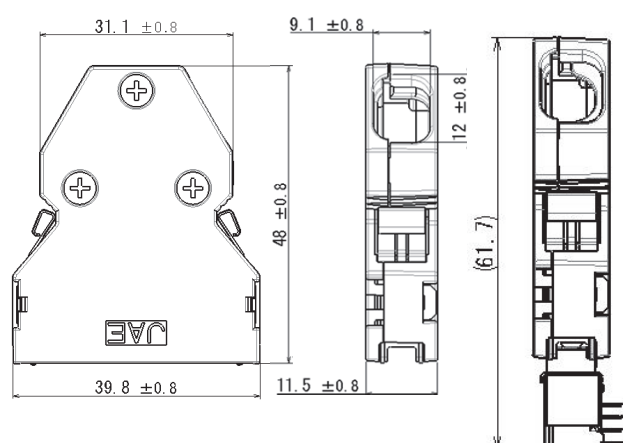
Mated Condition
