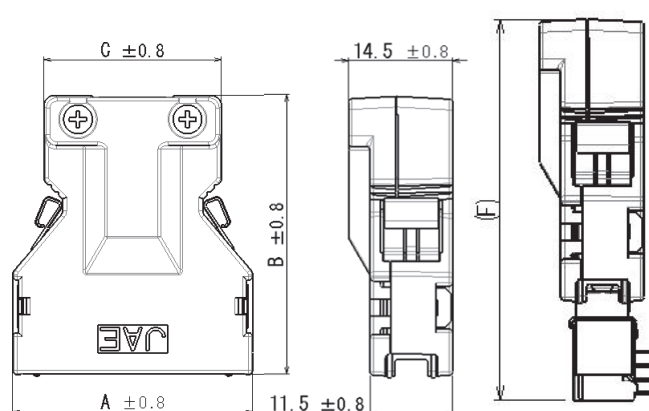
Mated Condition
