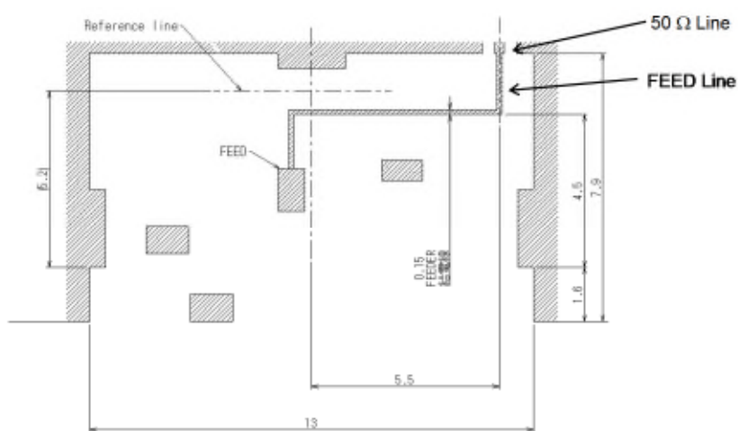
Reference board pattern (board thickness: 1.6 mm)
