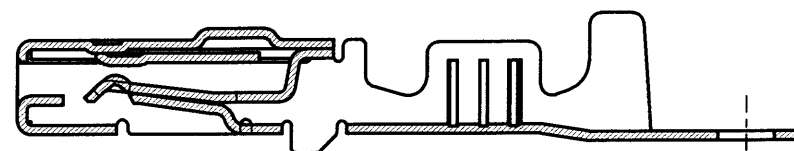
SECT. B-B (SCALE 5:1)
