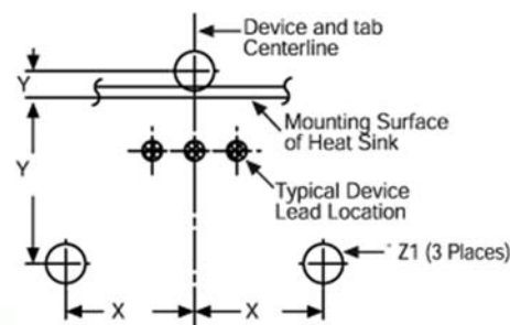
Mounting Details:
