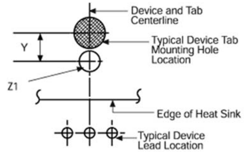
Mounting Details:
