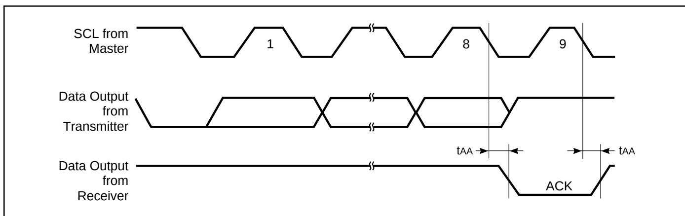
Figure 2. Output Acknowledge
