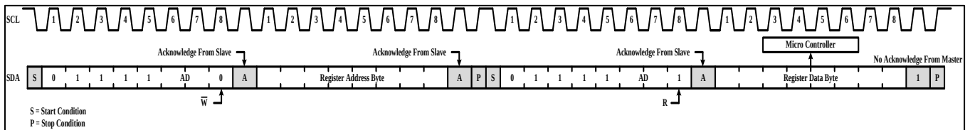
Figure 5 Reading from IS32SE5117
