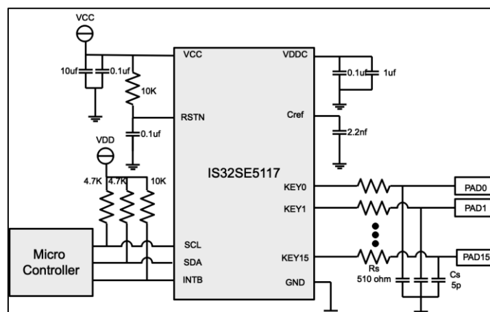
Figure 1 Typical Application Circuit (Wettable flank QFN-24)
