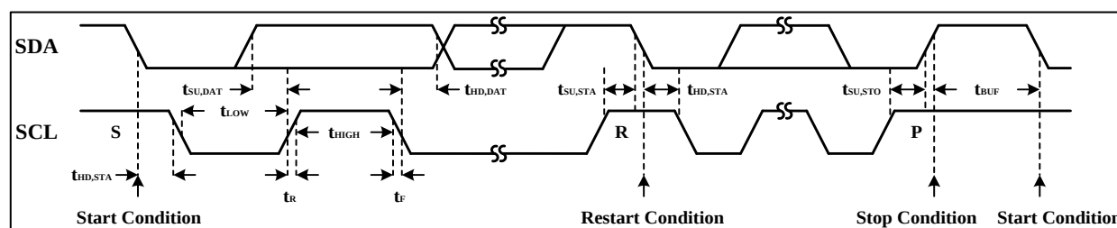
Figure 2 Interface Timing
