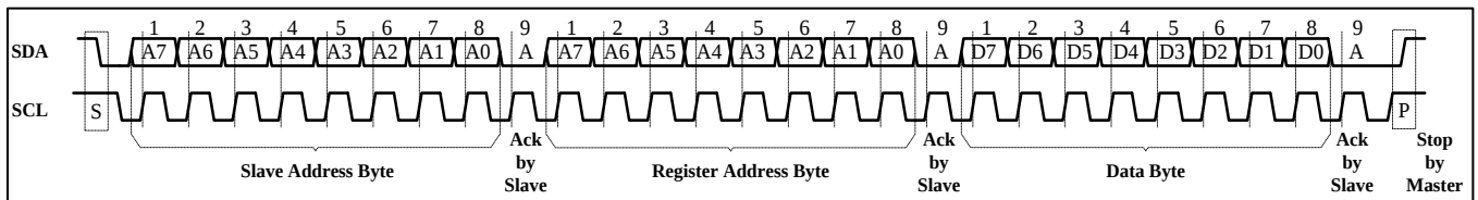
Figure 4 Writing to IS32SE5117
