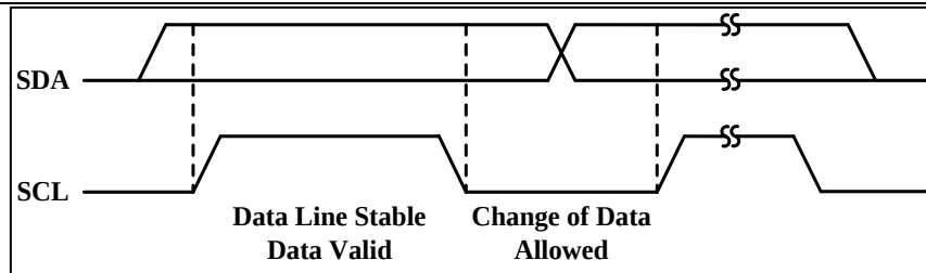
Figure 3 Bit Transfer
