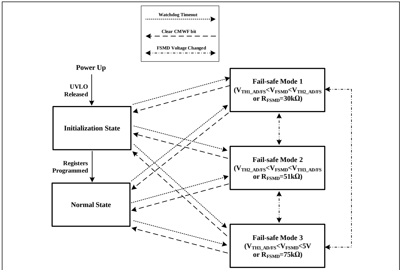
Figure 23 Operation States
