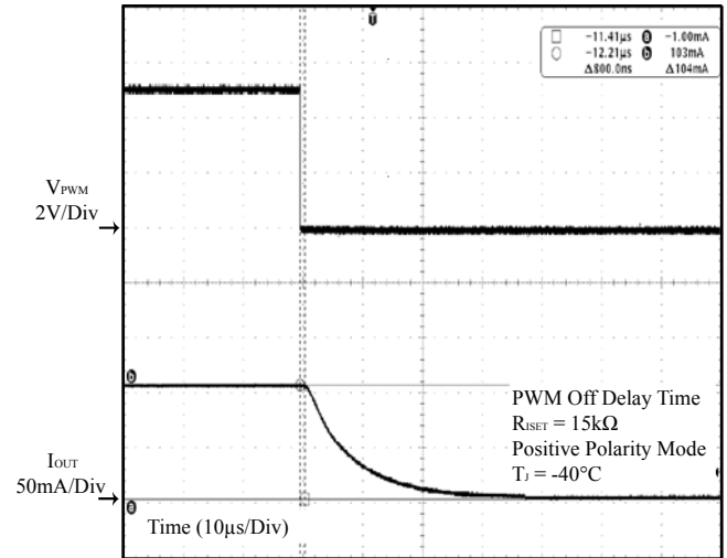
Figure 34 PWM Off Delay Time
