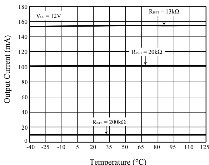
Figure 11 I_{OUT} vs. T_J
