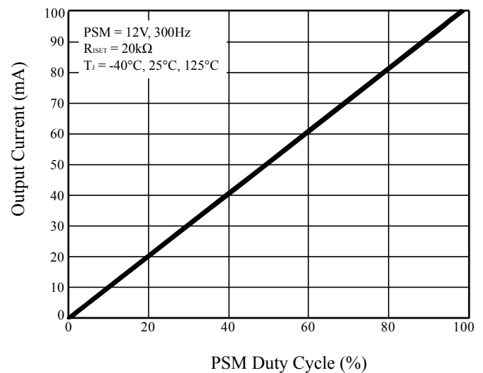
Figure 31 PSM Dimming at 300Hz
