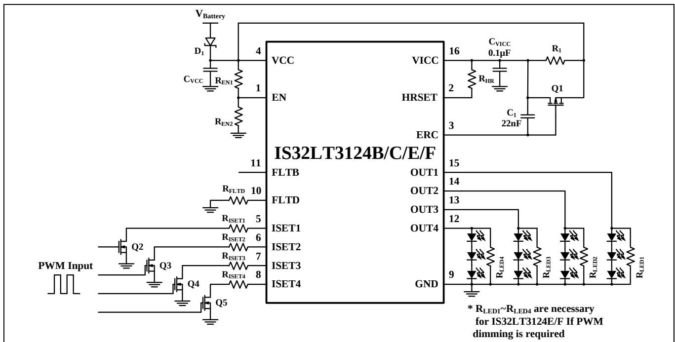
Figure 4 Typical Application Circuit with Additional Switches driving R ISER Individual PWM Dimming (IS32LT3124B/C/E/F only) When PWM Generator is Far Away from Device
