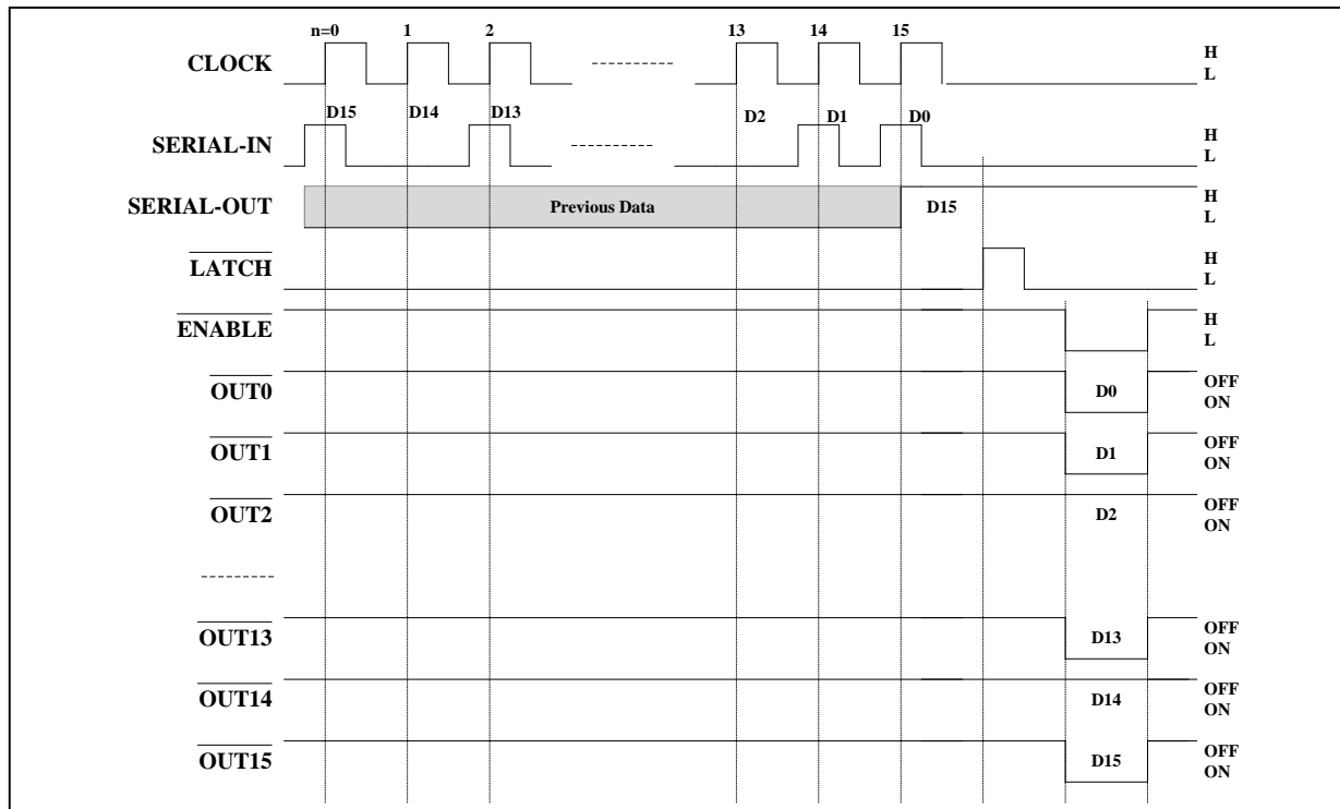
Figure 3 Timing Diagram
