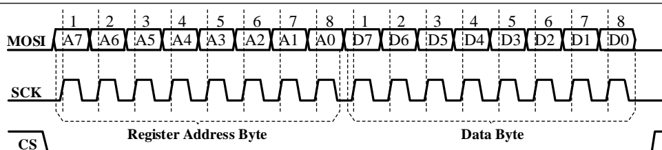
Figure 5 SPI writing to IS32FL3265B (Typical)
