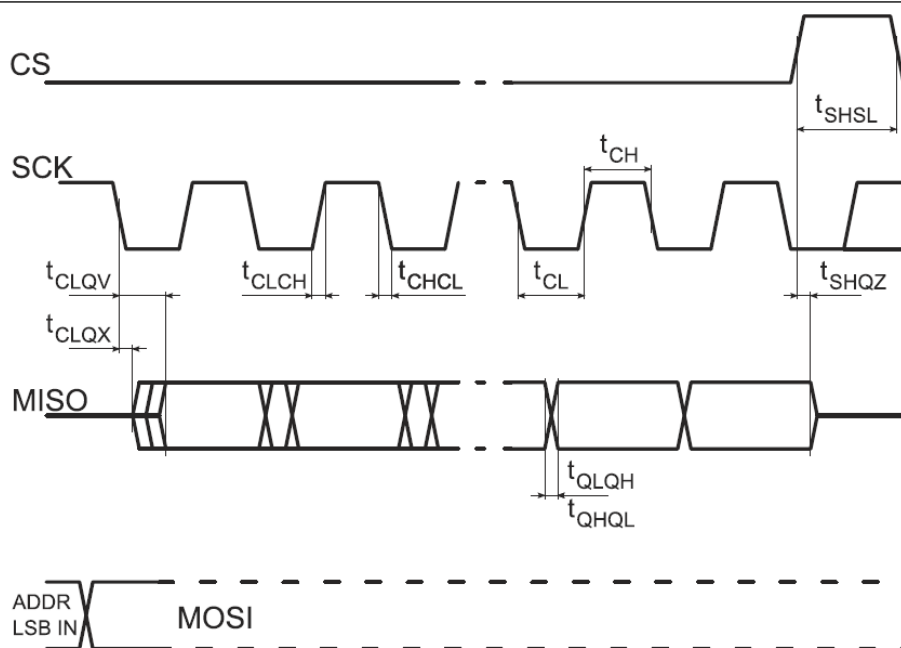
Figure 4 SPI Input Timing
