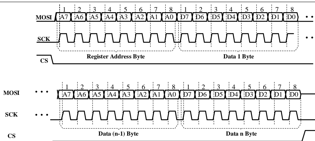
Figure 6 SPI writing to IS32FL3265B (Automatic Address Increment)
