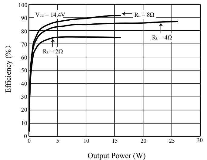
Figure 9 Efficiency vs. Output Power
