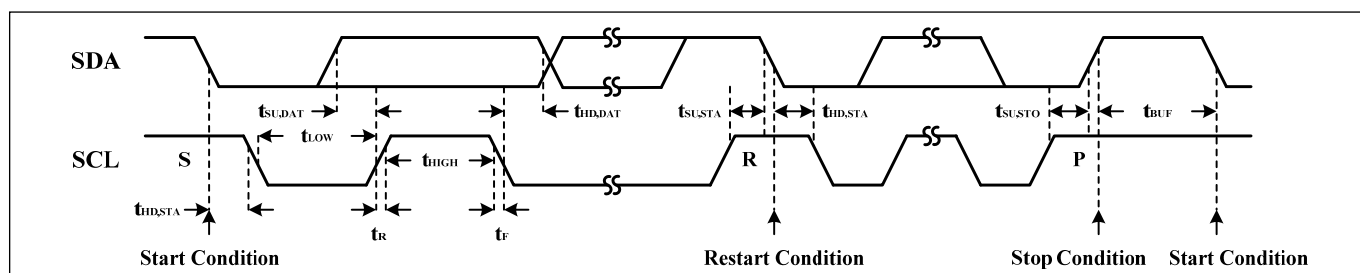
Figure 12 Interface Timing
