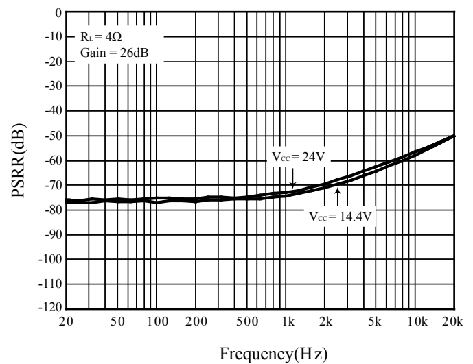
Figure 11 PSRR
