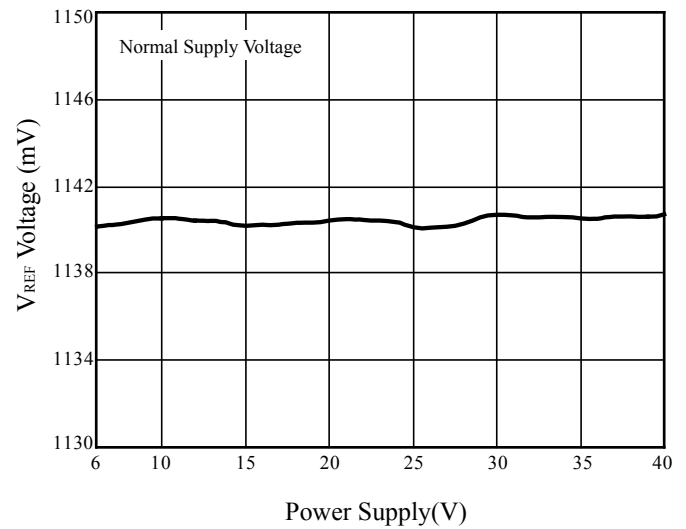
Figure 9 V_{REF} vs. Power Supply (Normal Supply Voltage)
