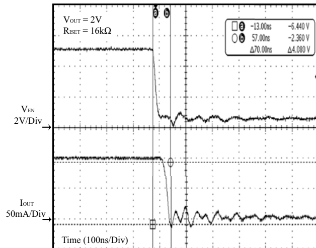
Figure 22 Shut Down
