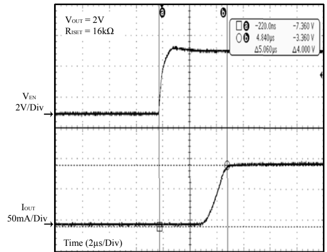
Figure 42 Start Up
