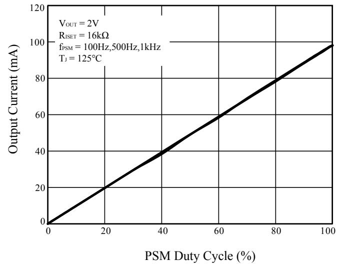
Figure 17 Output Current vs. PSM Duty Cycle
