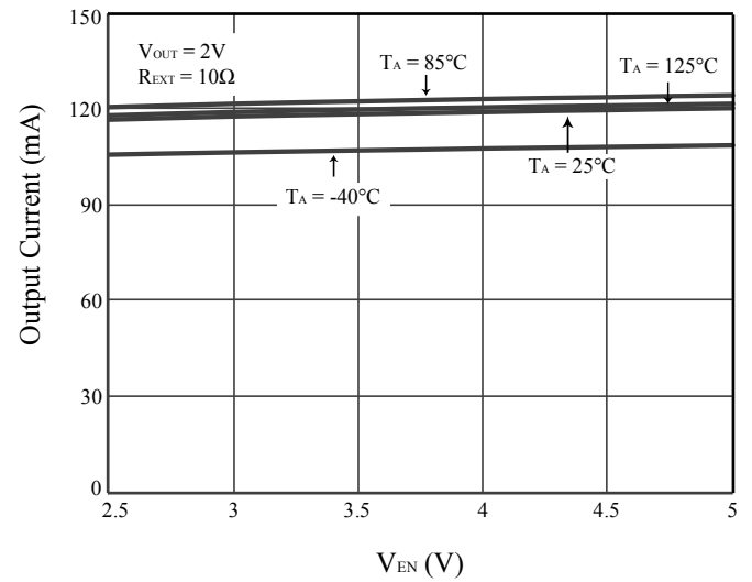
Figure 26 I_{OUT} vs. V_{EN}
