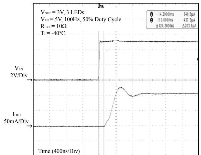
Figure 32 V_{EN} vs. I_{OUT} Delay and Rising Edge
