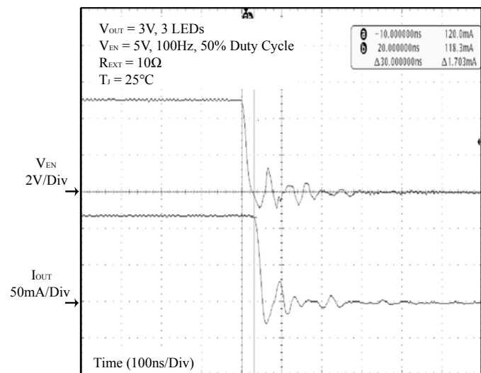
Figure 36 V_{EN} vs. I_{OUT} Delay and Falling Edge
