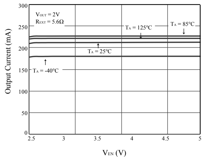
Figure 13 I_{OUT} vs. V_{EN}
