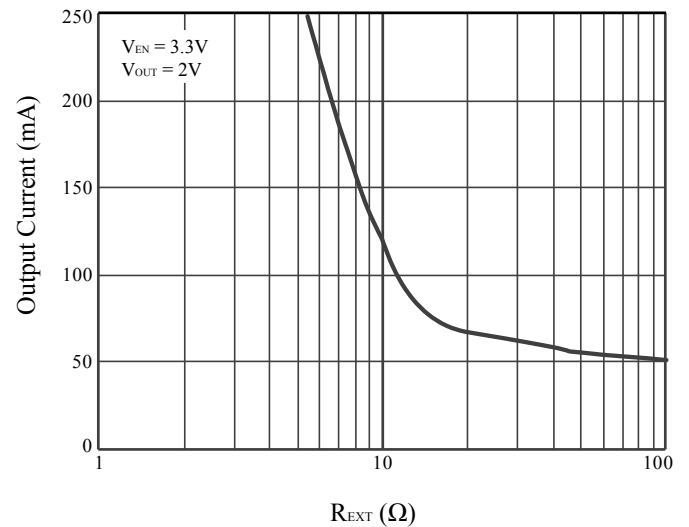
Figure 30 I_{OUT} vs. R_{EXT}
