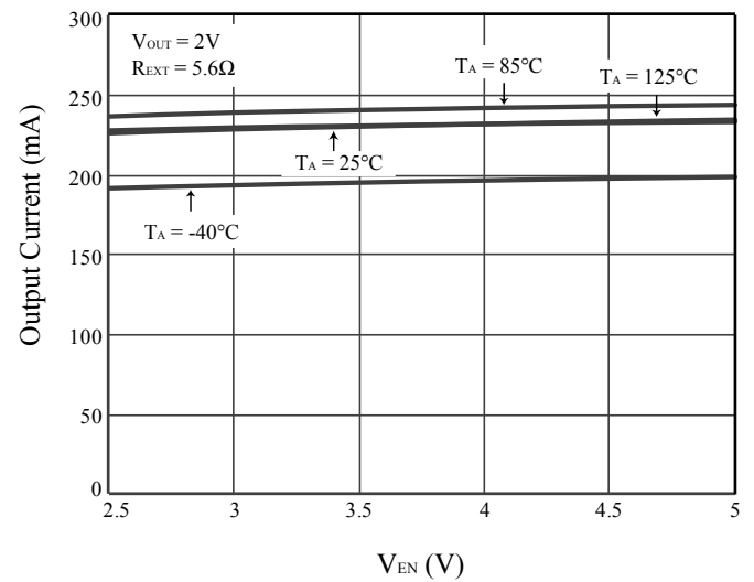
Figure 28 I_{OUT} vs. V_{EN}
