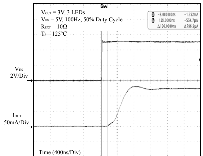
Figure 34 V_{EN} vs. I_{OUT} Delay and Rising Edge
