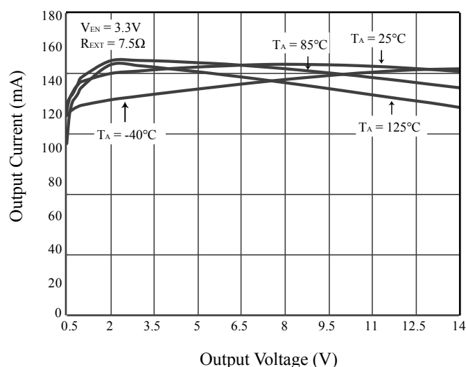
Figure 20 I_{OUT} vs. V_{OUT}
