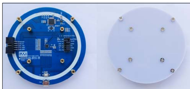
Figure 1: Photo of IS31FL3746A Evaluation Board
