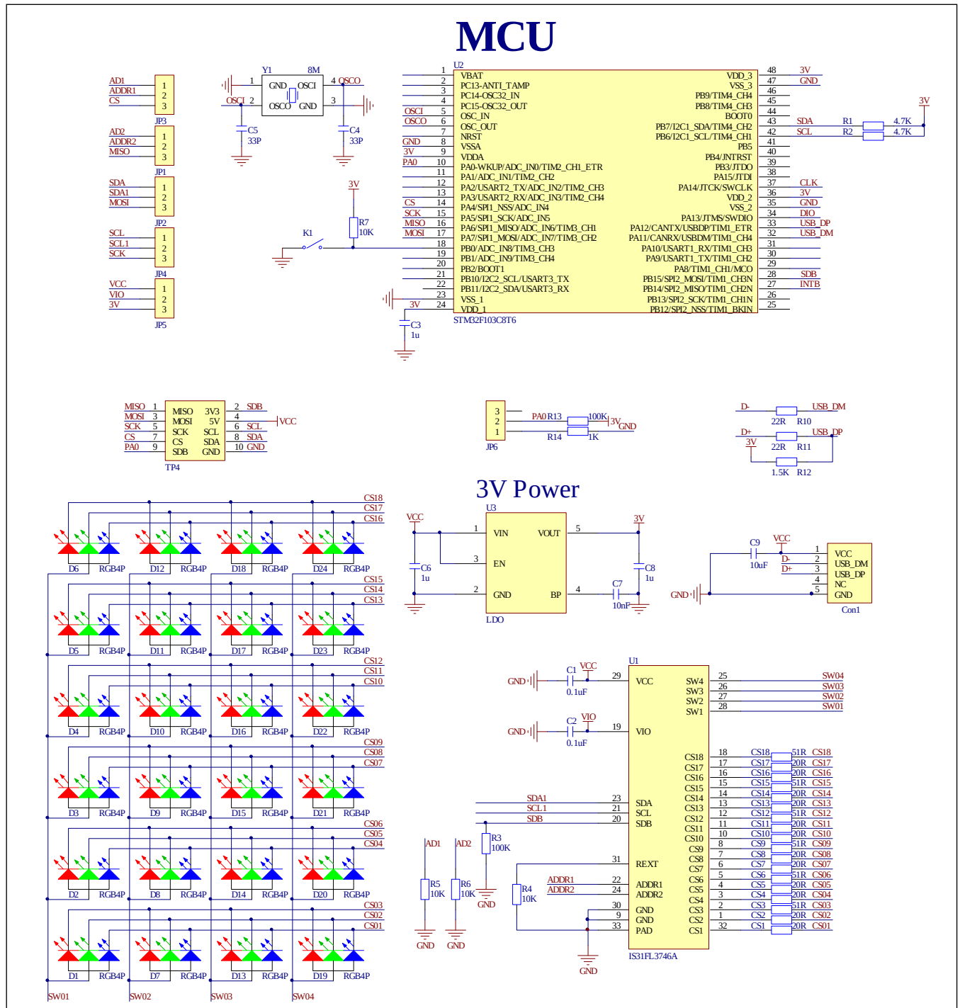
Figure 3: IS31FL3746A Application Schematic
