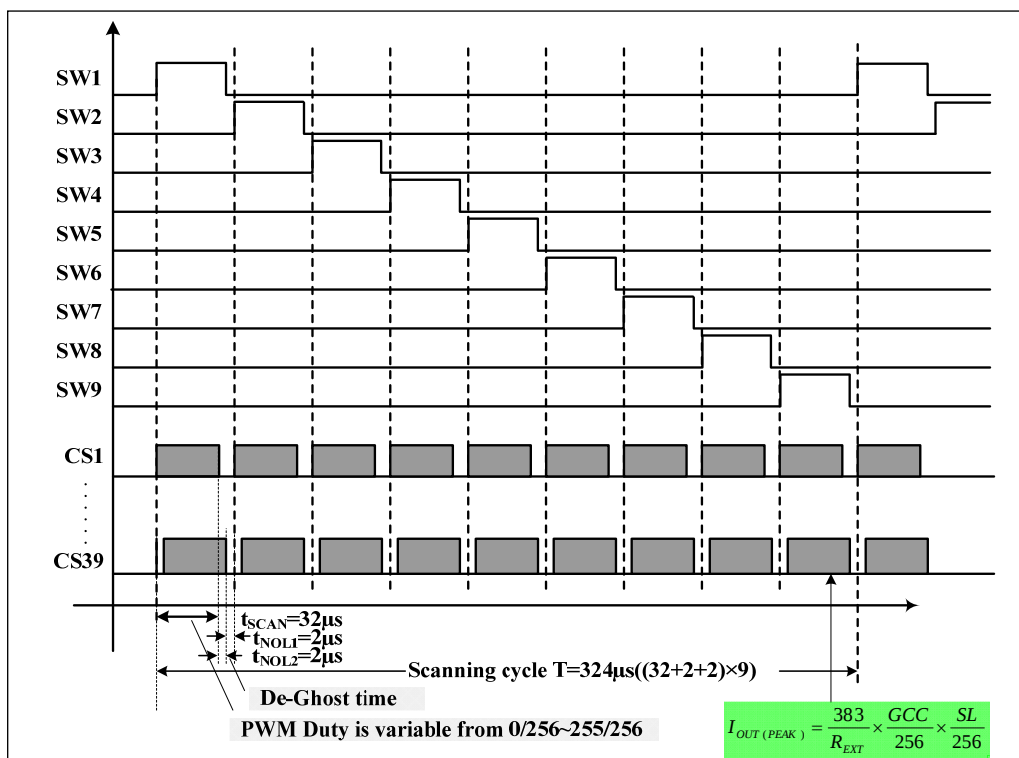
Figure 11 Scanning Timing
