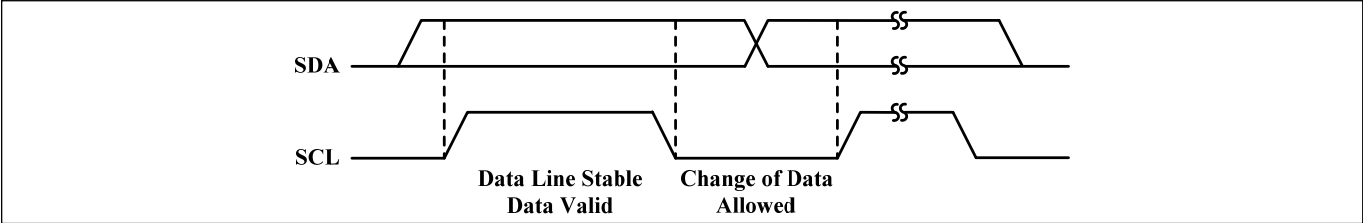
Figure 5 Bit Transfer
