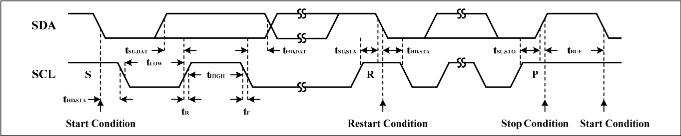
Figure 4 Interface Timing
