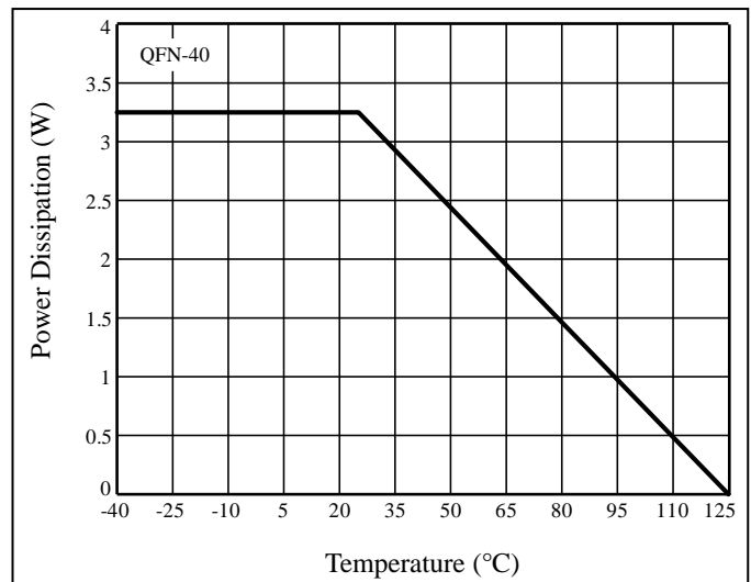
Figure 17 Dissipation Curve
