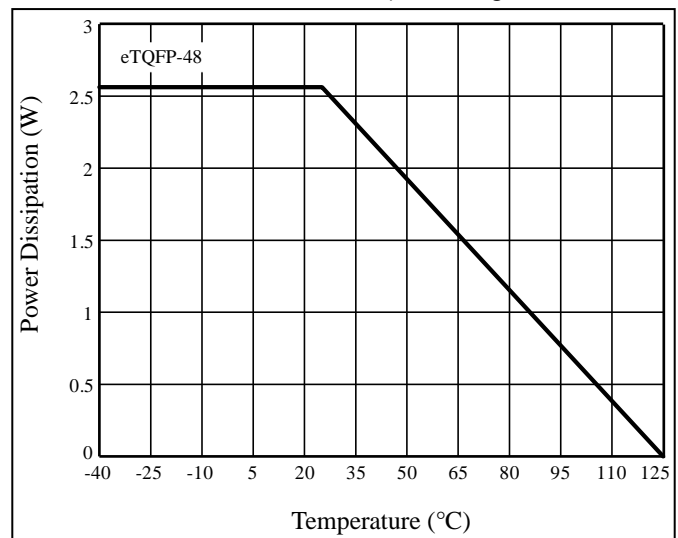
Figure 17 Dissipation Curve
