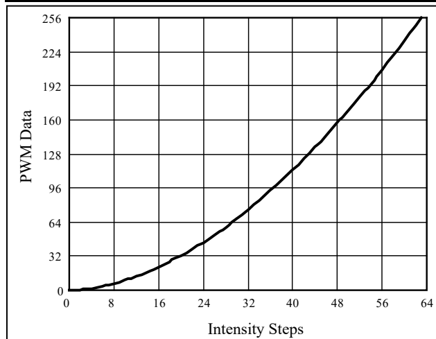
Figure 9 Gamma Correction (64 Steps)
