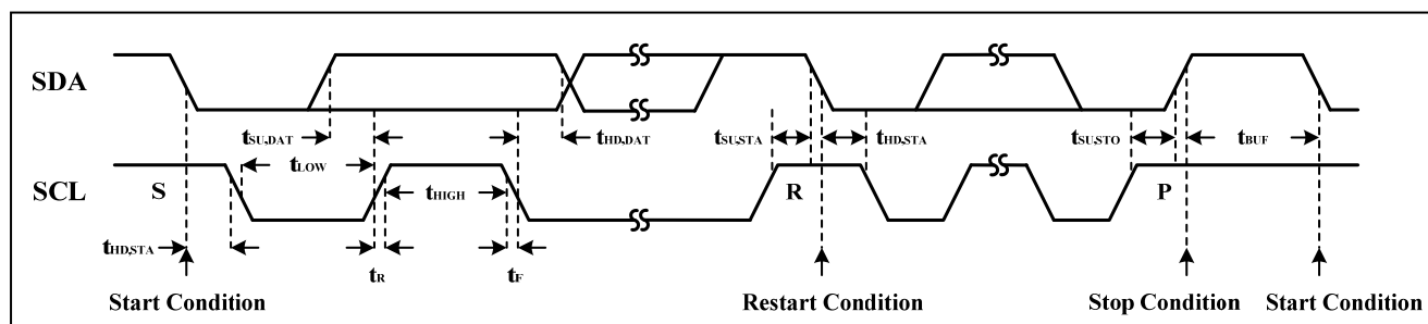
Figure 3 Interface timing
