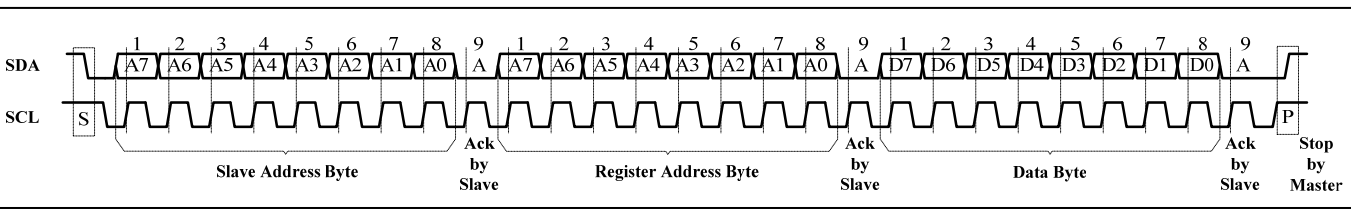
Figure 5 Writing to IS31FL3216A (Typical)
