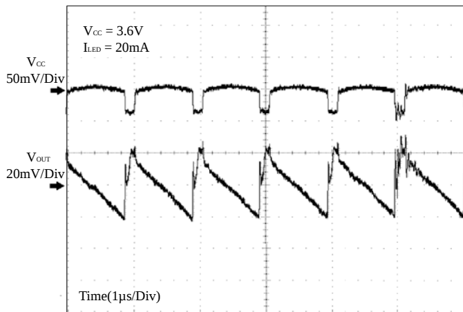
Figure 9 Ripple Voltage
