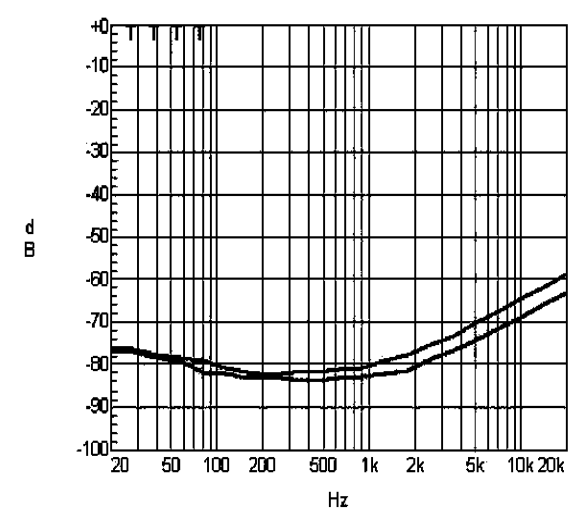
Figure 19 PSRR vs. Freq SE mode, 3V, 32Ohm, 200mVpp Input terminated
