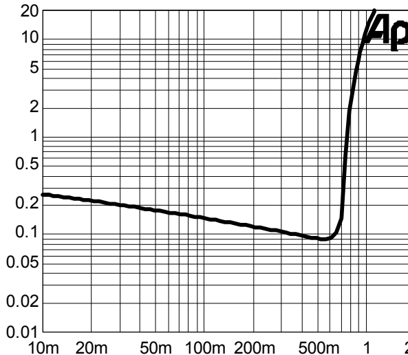
Figure 7 THD+N vs. Output Power BTL mode, 3V, 40hm, f=1kHz
