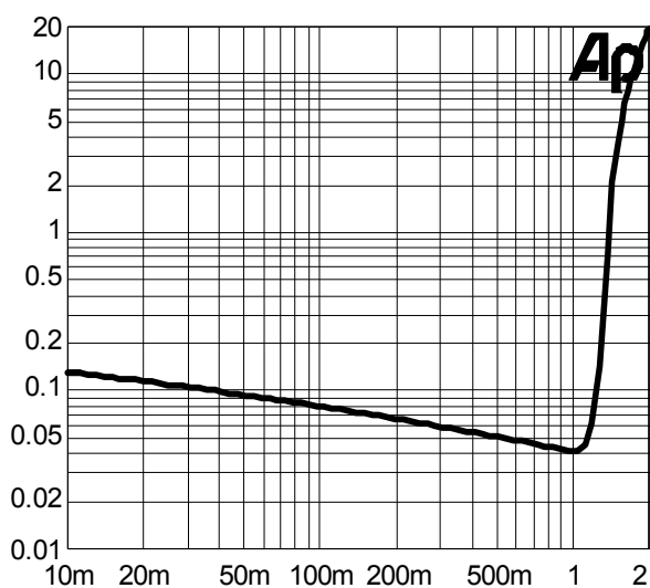
Figure 2 THD+N vs. Output Power 5V, 80hm, BTL at f=1kHz
