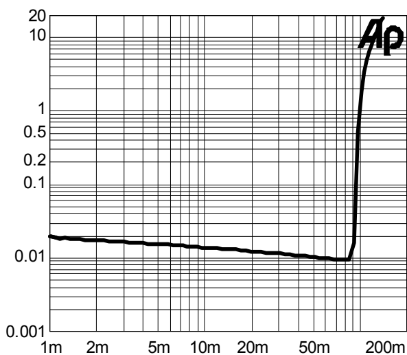
Figure 4 THD+N vs. Output Power SE mode, 5V, 320hm, f=1kHz
