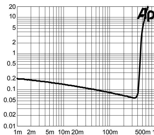
Figure 3 THD+N vs. Output Power 3V, 80hm, BTL at f=1kHz
