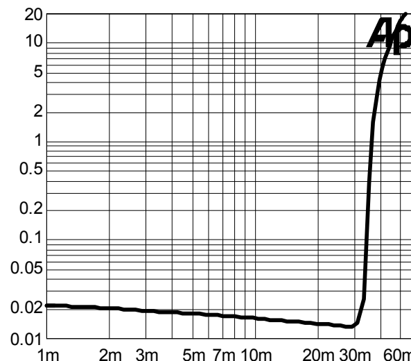
Figure 5 THD+N vs. Output Power SE mode, 3V, 320hm, f=1kHz
