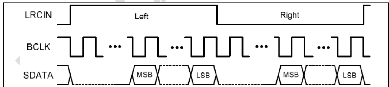
Figure 7 Right-Alignment
