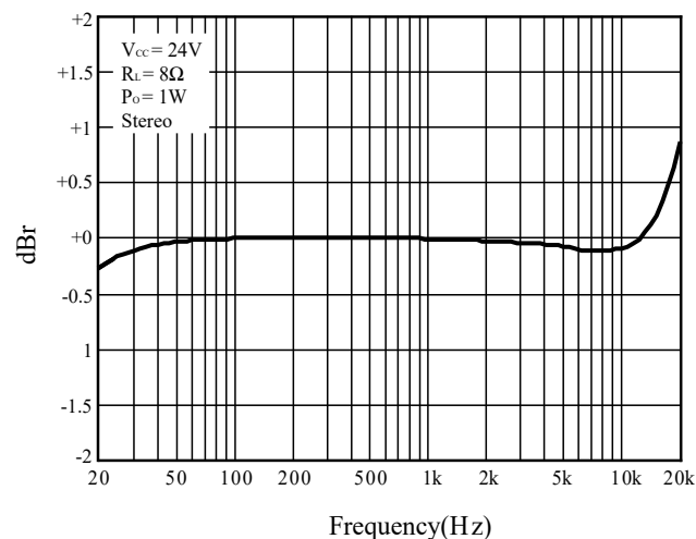
Figure 21 Frequency Response
