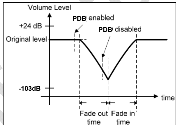
Figure 31 Power Down Timing Diagrams
