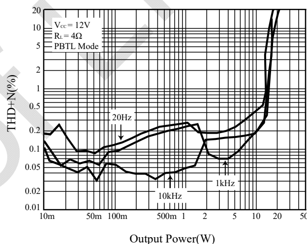
Figure 19 THD+N vs. Output Power
