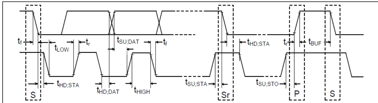
Figure 4 I2C Timing
