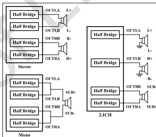
Figure 32 Output Configurations
