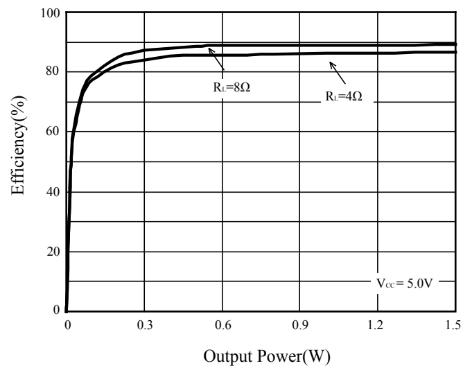
Figure 9 Efficiency
