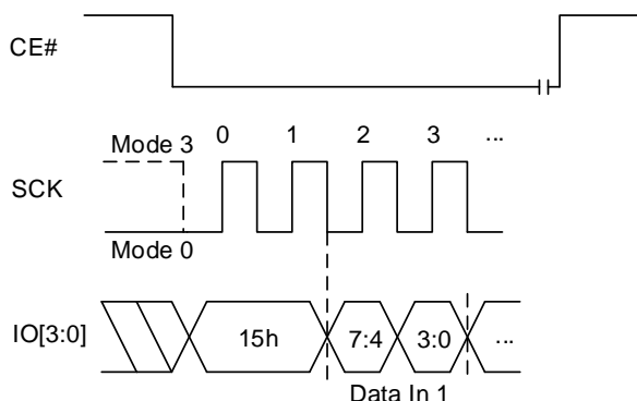
Figure 8.106 WRABR Sequence In QPI Mode
